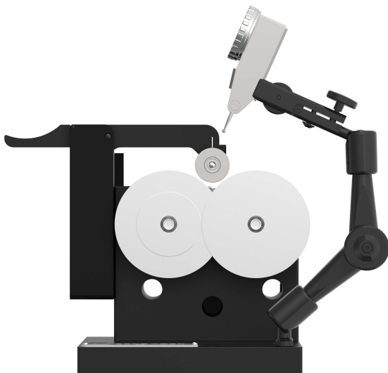
Run-out tester RPG 0825 AL Front view
